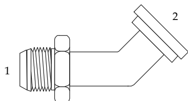
(1) Male Tube (2) C 61 Flange
