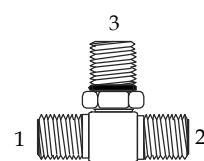
(1)(2) Male Face Seal (3) Male Adj. ORB
