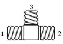
(1)(2) Male Face Seal (3) Male NPT
