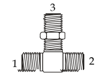
(1)(2) Male Face Seal (3) Face Seal Bulkhead
