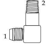
(1) Male JIC (2) Male NPT Long
