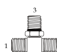
(1)(2) Male Face Seal (3) Male Adj. ORB
