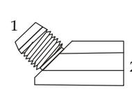
(1) Male JIC (2) Female NPT
